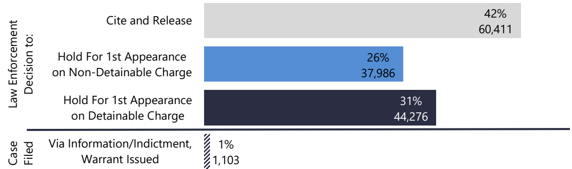
Figure 2A. Law Enforcement Decision to Cite and Release or Hold for First Appearance Hearing - Criminal Cases Filed in the Circuit Court of Cook County: 09/18/2023 - 12/06/2025 (n=143,776)
