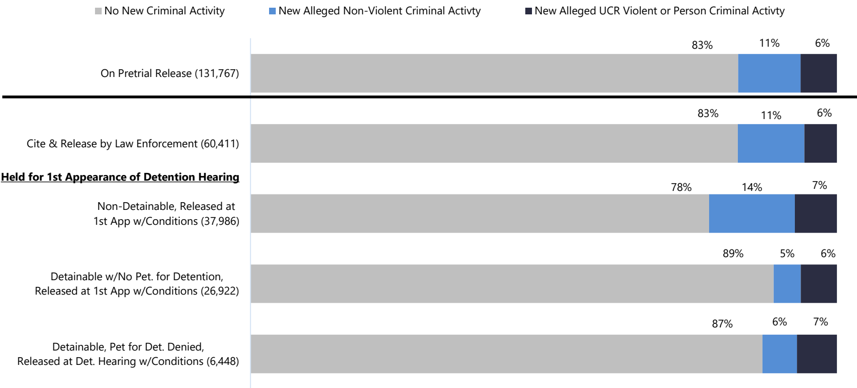
Figure 6. Community Safety Rate for Criminal Cases Filed by PFA Stage of Pretrial Release: 09/18/2023 - 12/06/2025
